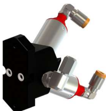
Bypass 2 valves, with solvent injection
