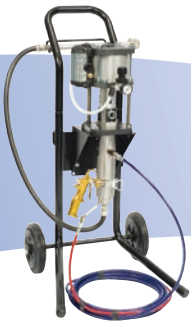
MXL1231PU-C-ACG – cart mounted AAA outfit
