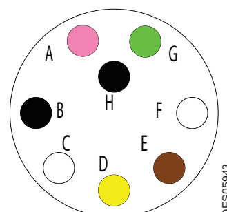
Plug side GNM 6080
