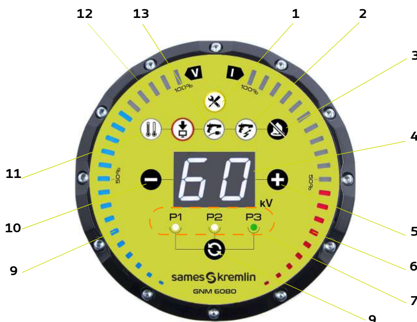
Front face of the GNM 6080 control module
