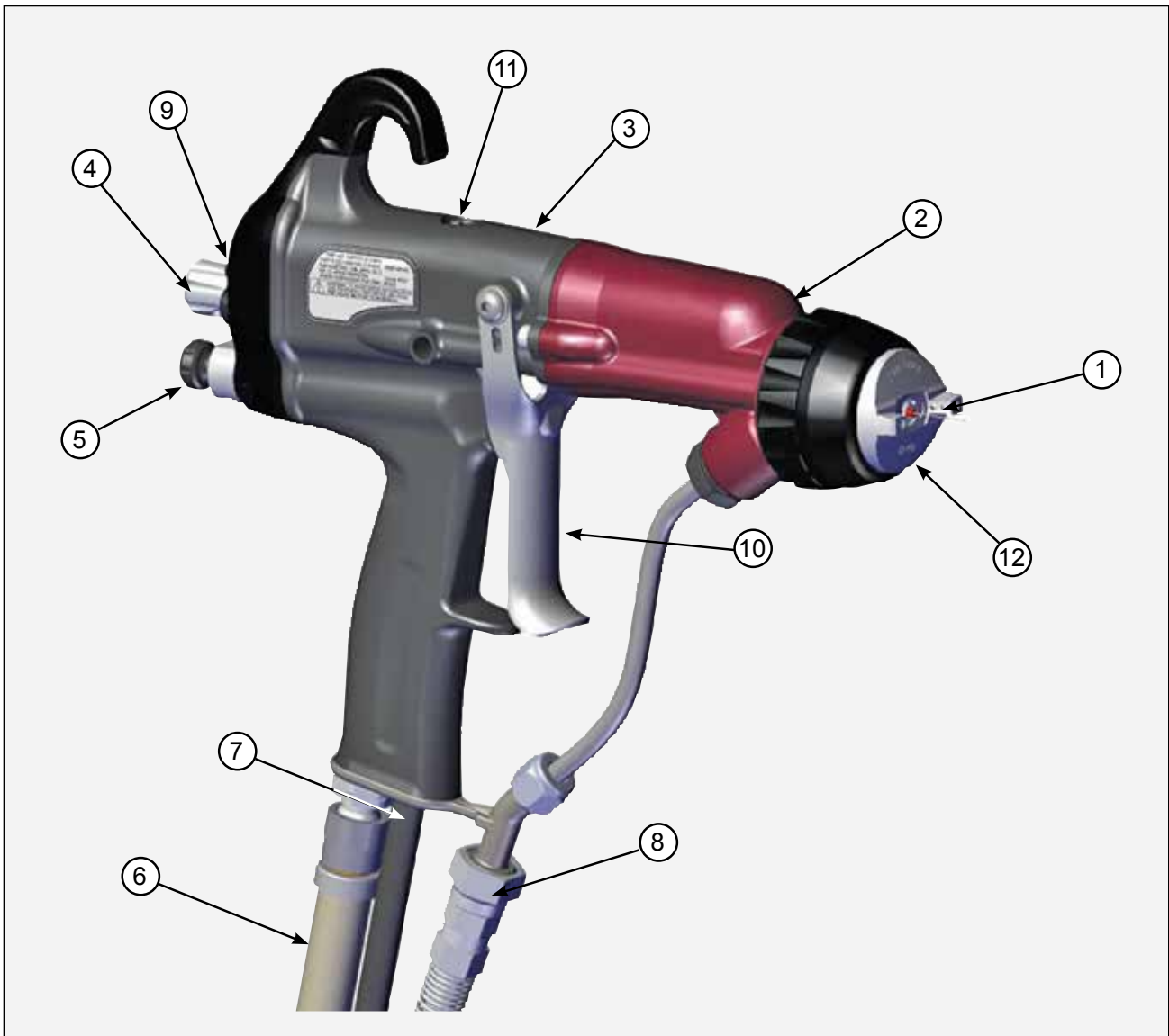
Figure 1: Ransflex Indirect Charge Waterborne Electrostatic Spray Applicator 80445
