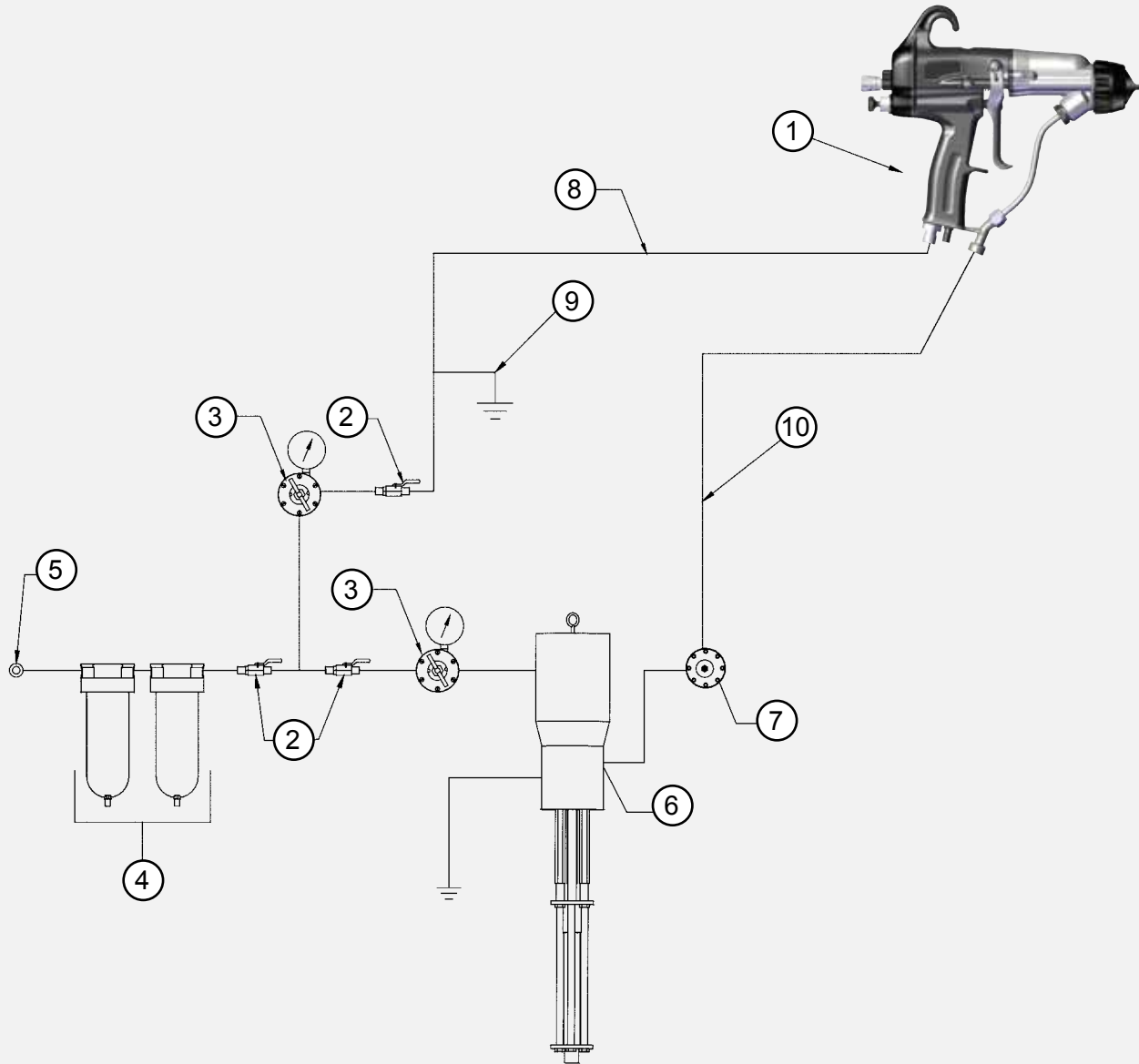
Figure 2: Ransflex Installation for Waterbase Materials
