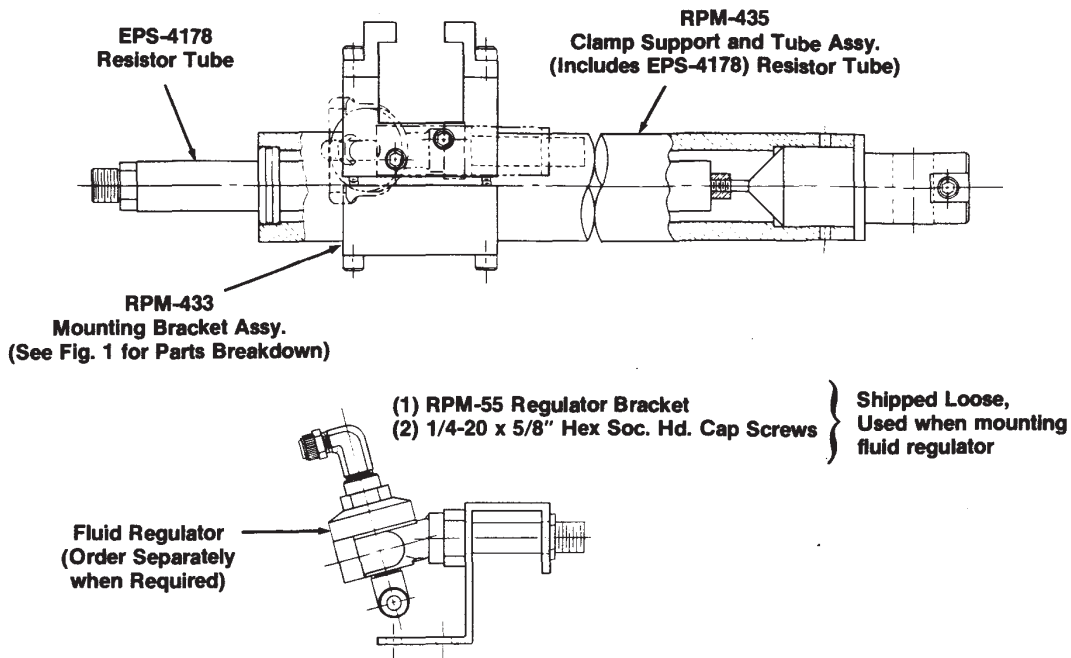
Figure 2: RPM-434 Support and Tube Assembly
