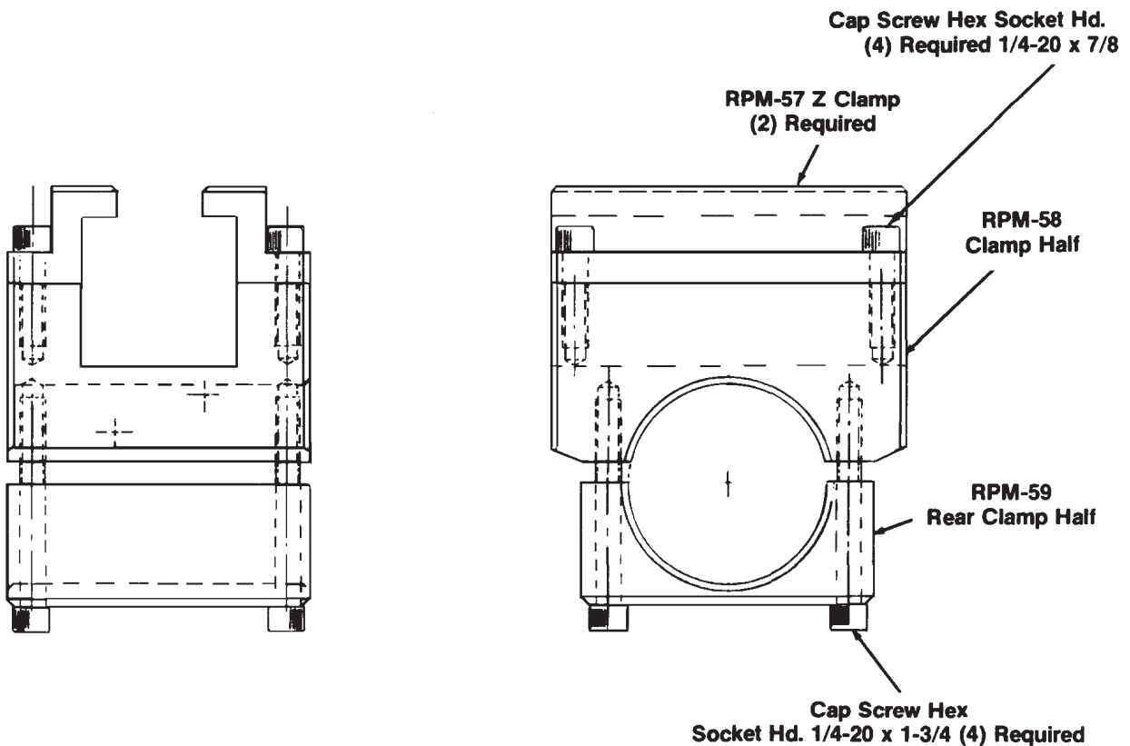
Figure 1: RPM-433 Mounting Bracket Assembly
