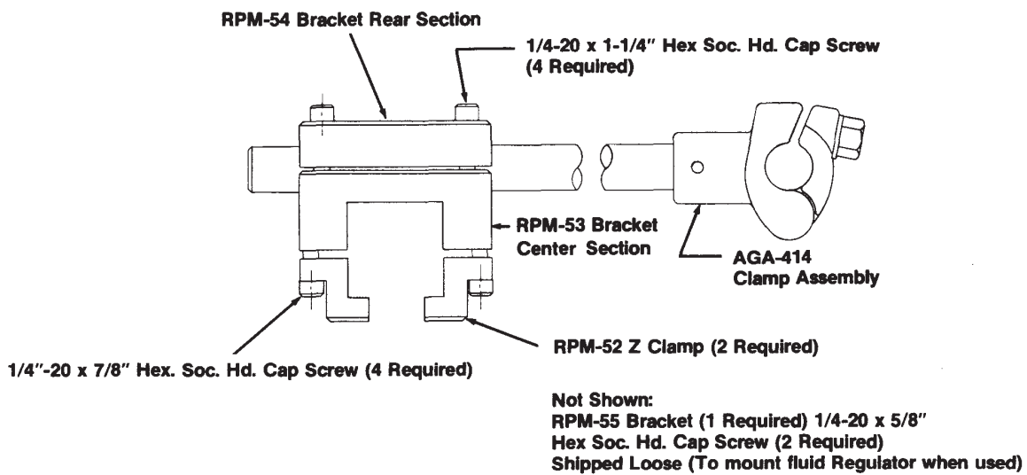
Figure 3: RPM-436 Mounting Bracket and Clamp Assembly
