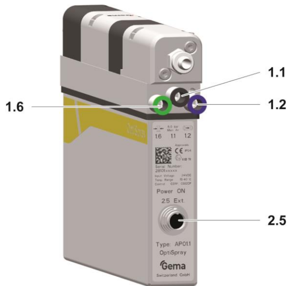
fig. 13: Connecting material
