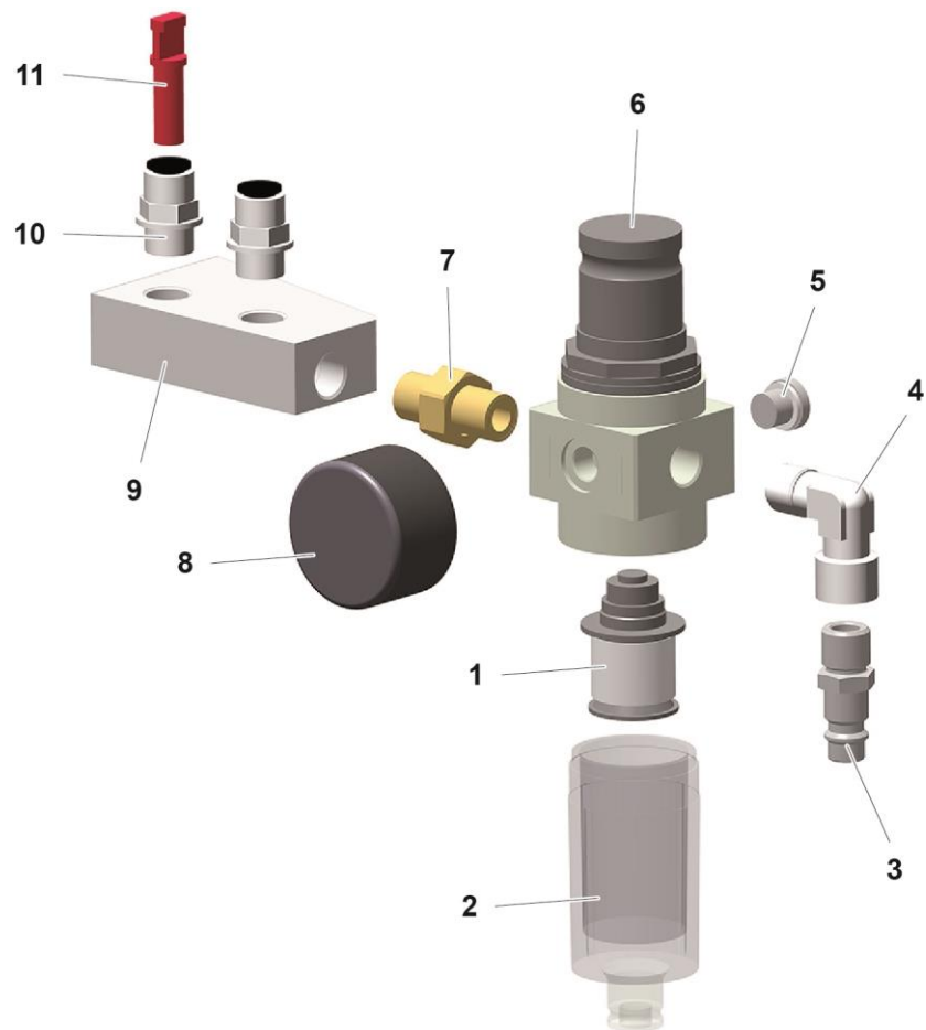
fig. 11: Pneumatic group
