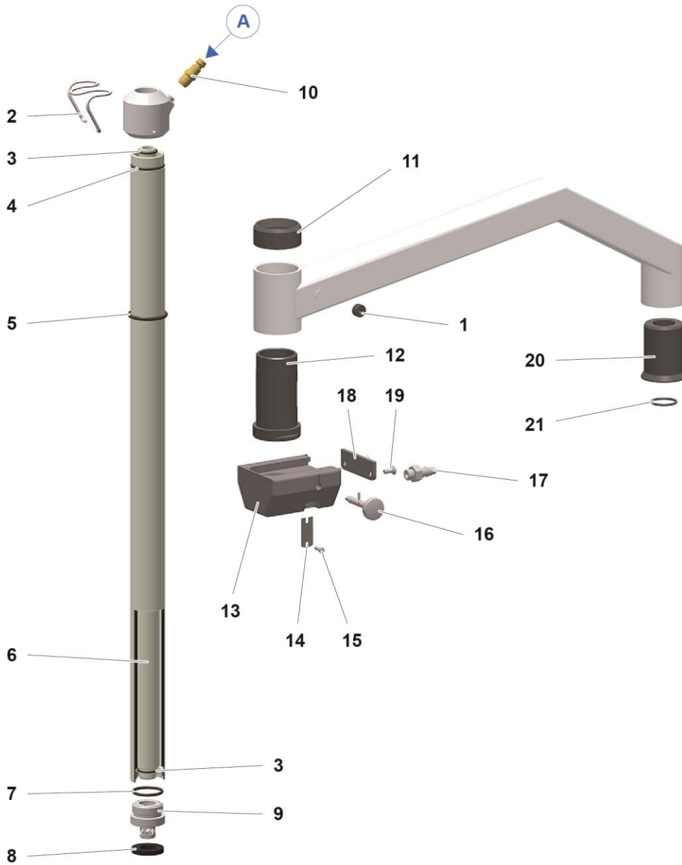
fig. 10: Fluidizing/suction tube – spare parts
