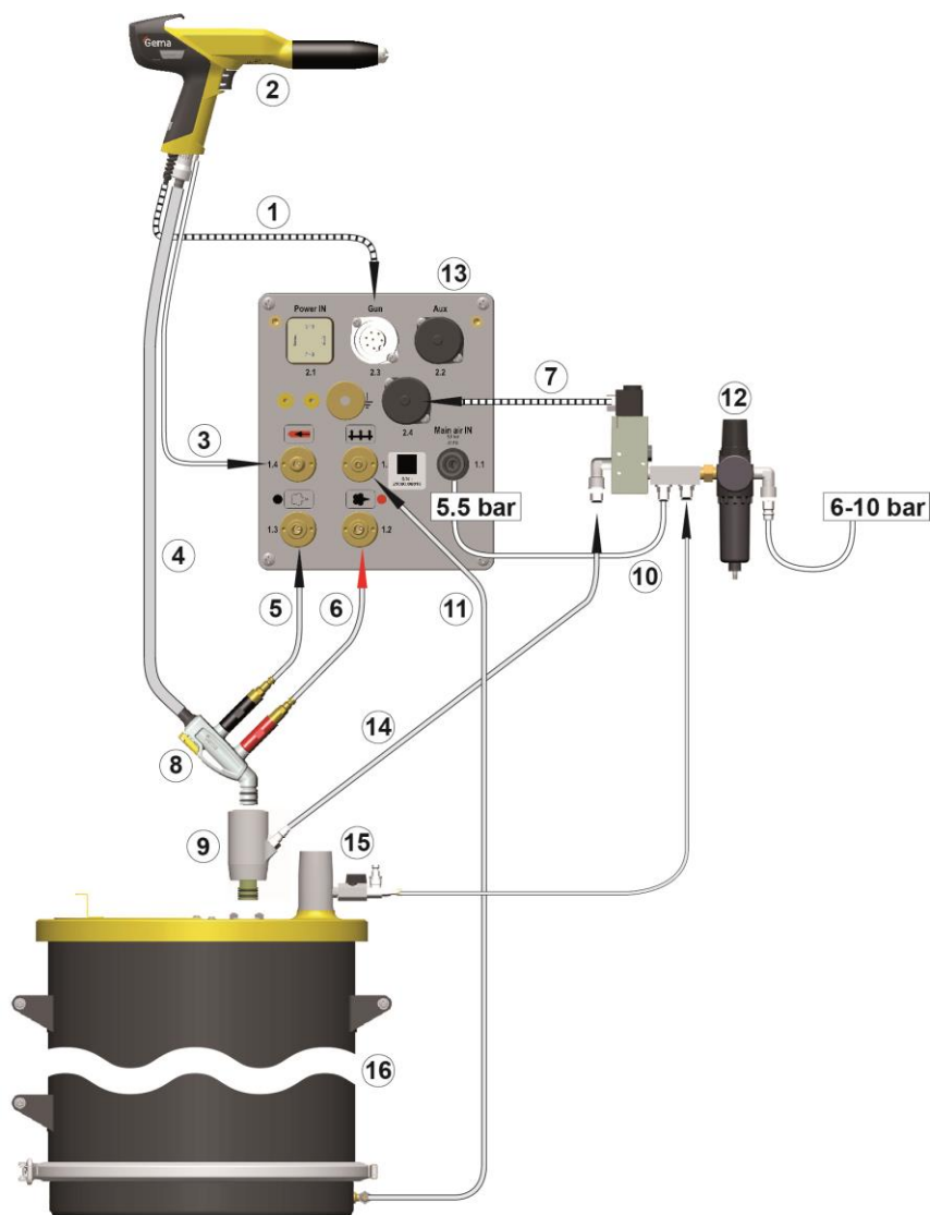
fig. 6: Connecting guide – overview
