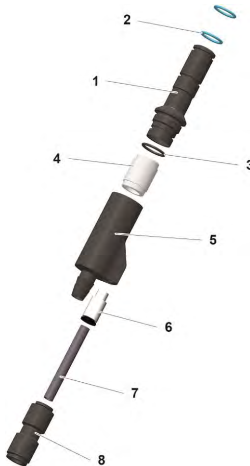
fig. 12: Diffuser (OptiSelect)
