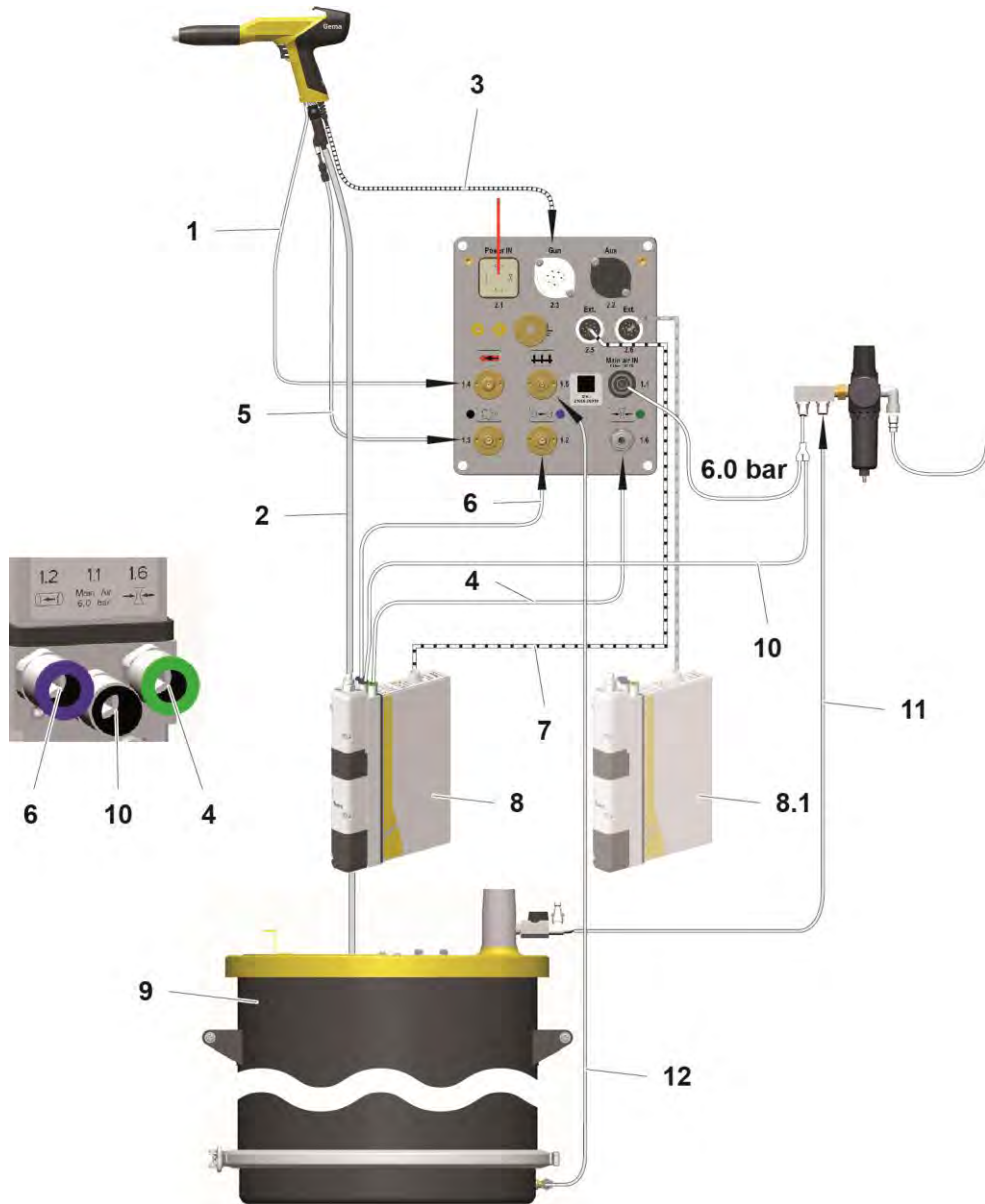
fig. 6: Connecting guide – overview
