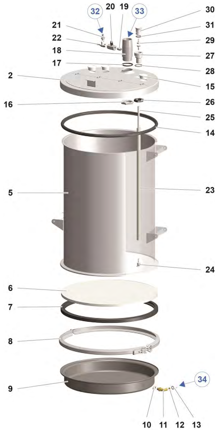
fig. 11: Powder hopper HF05-50 Spray
