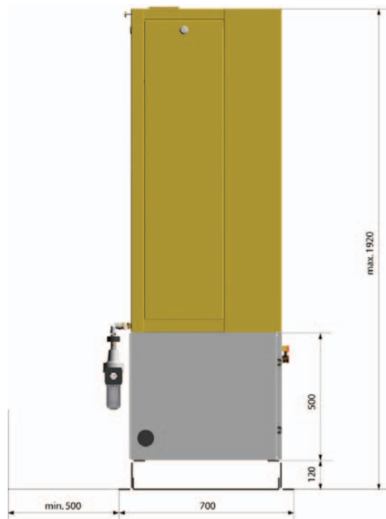
OptiFlex A2 Control system with CM-20 - assembly
