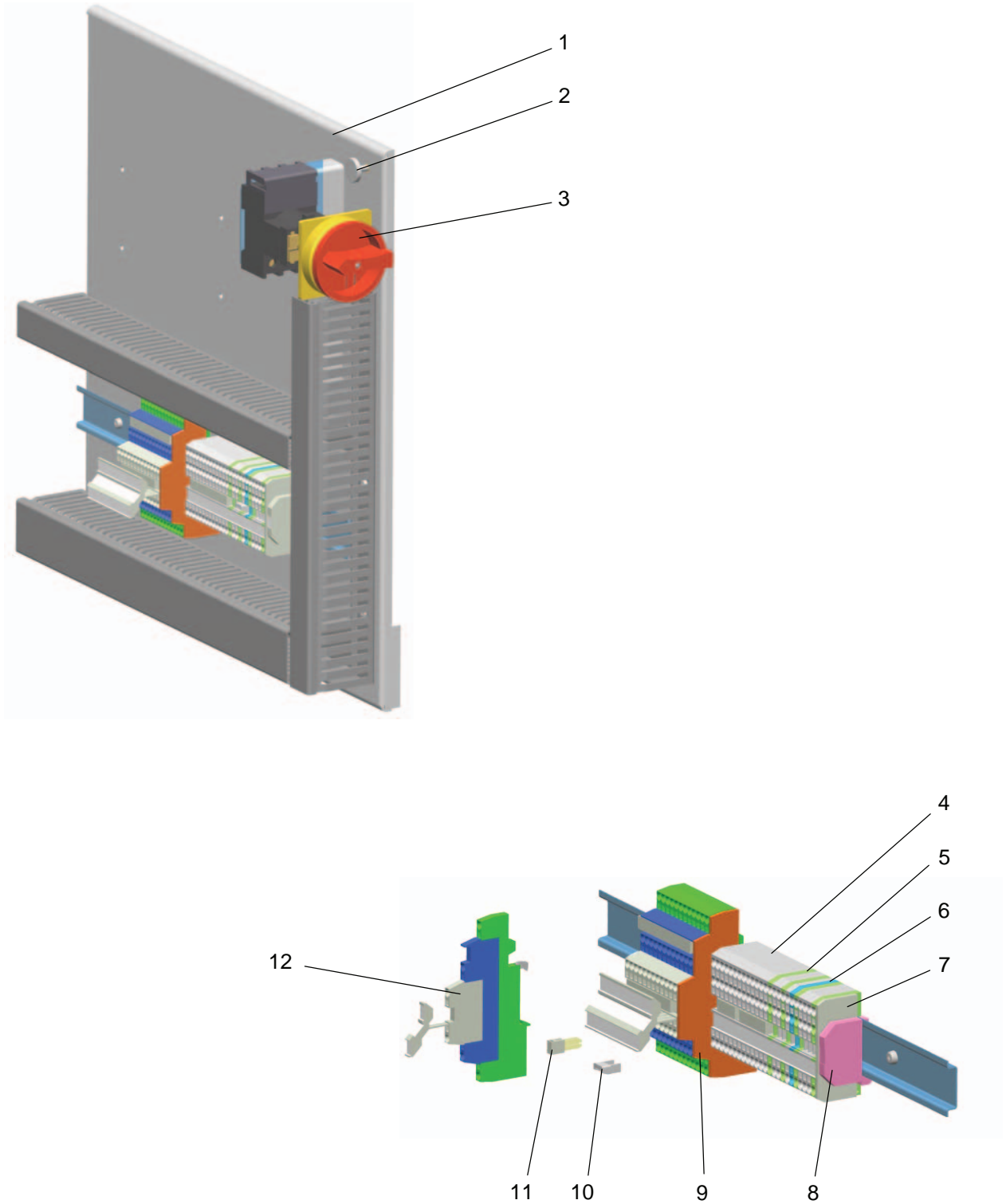
OptiFlex A2 - mounting plate
