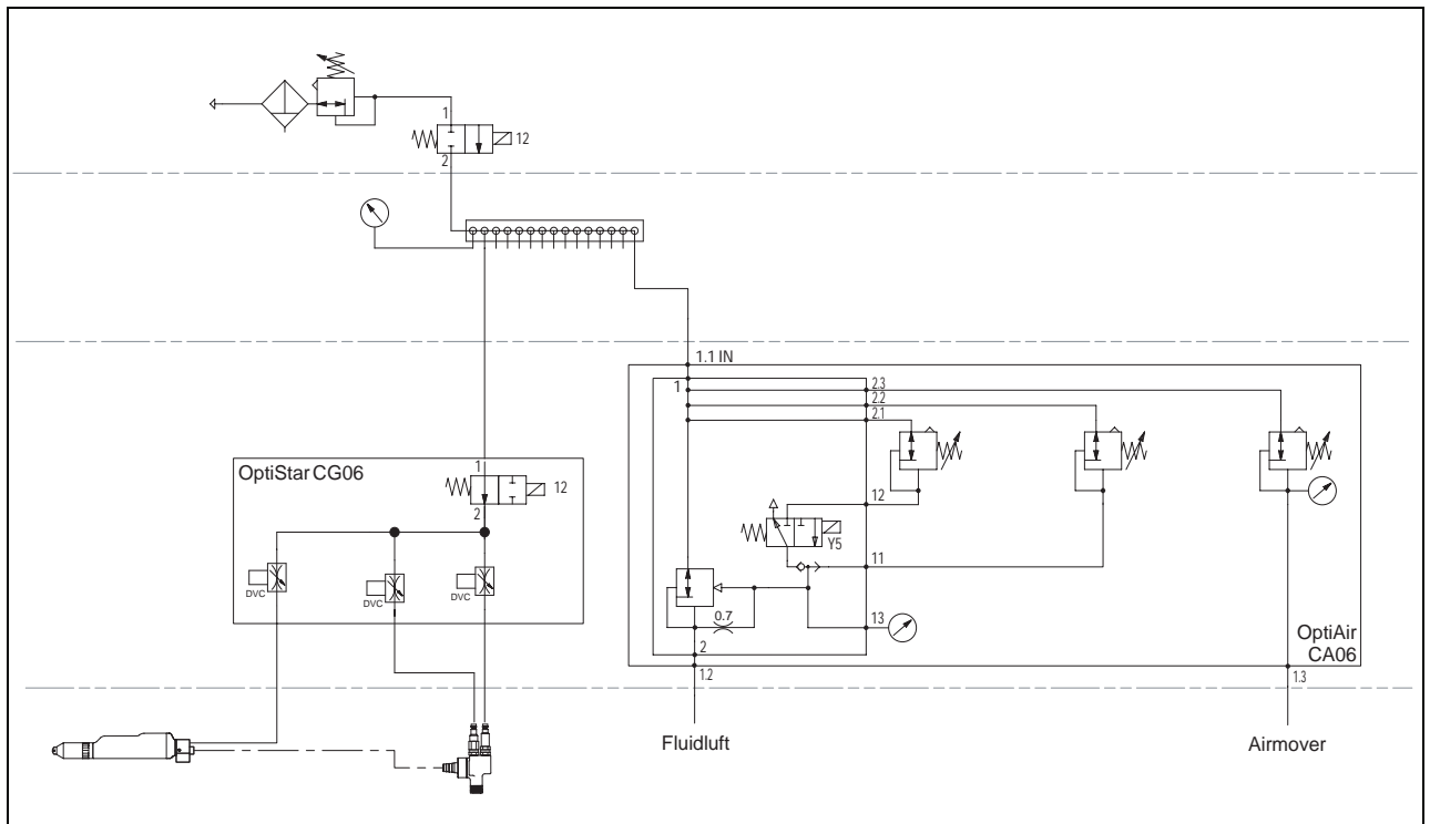
OptiFlex A2 Control system - pneumatical diagram
