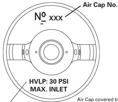
Figure 1 Air Cap
