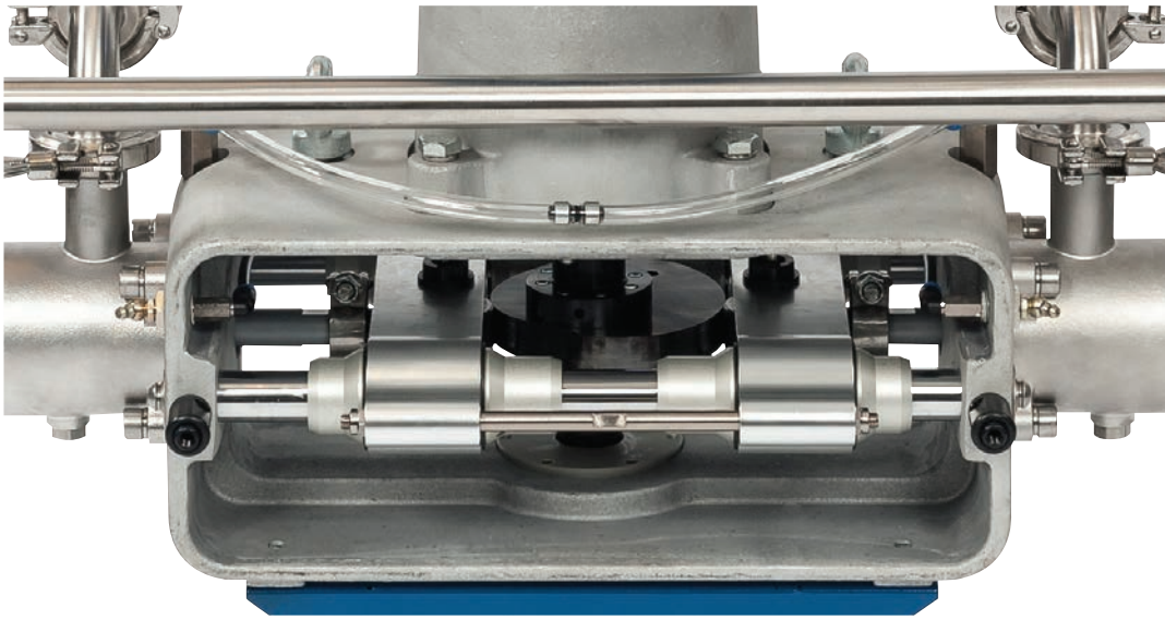
Asymmetric constant velocity cam.
